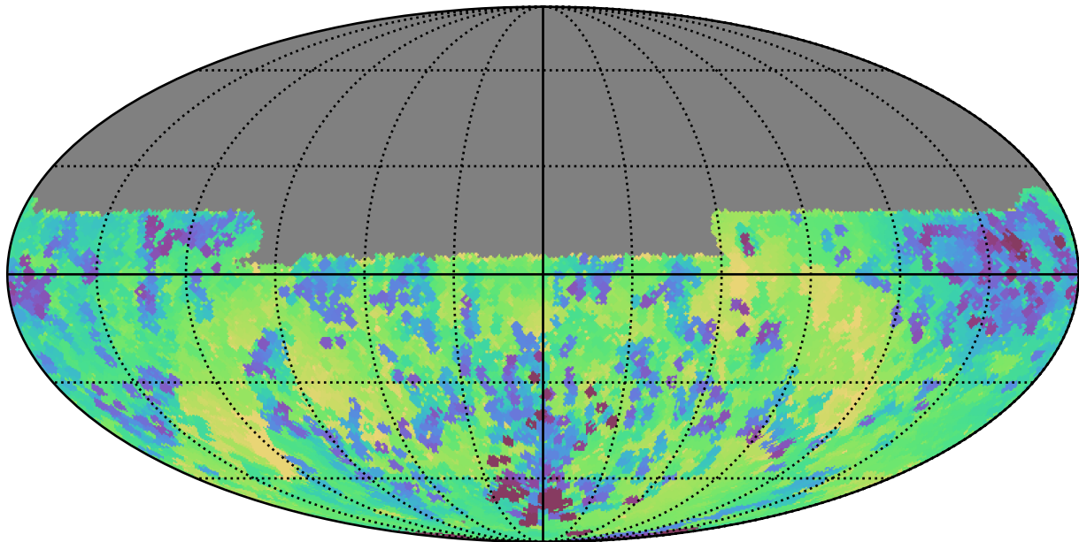
weather_cloudso2v3.4_10yrs Yr 1 y band: Min skyBrightness
