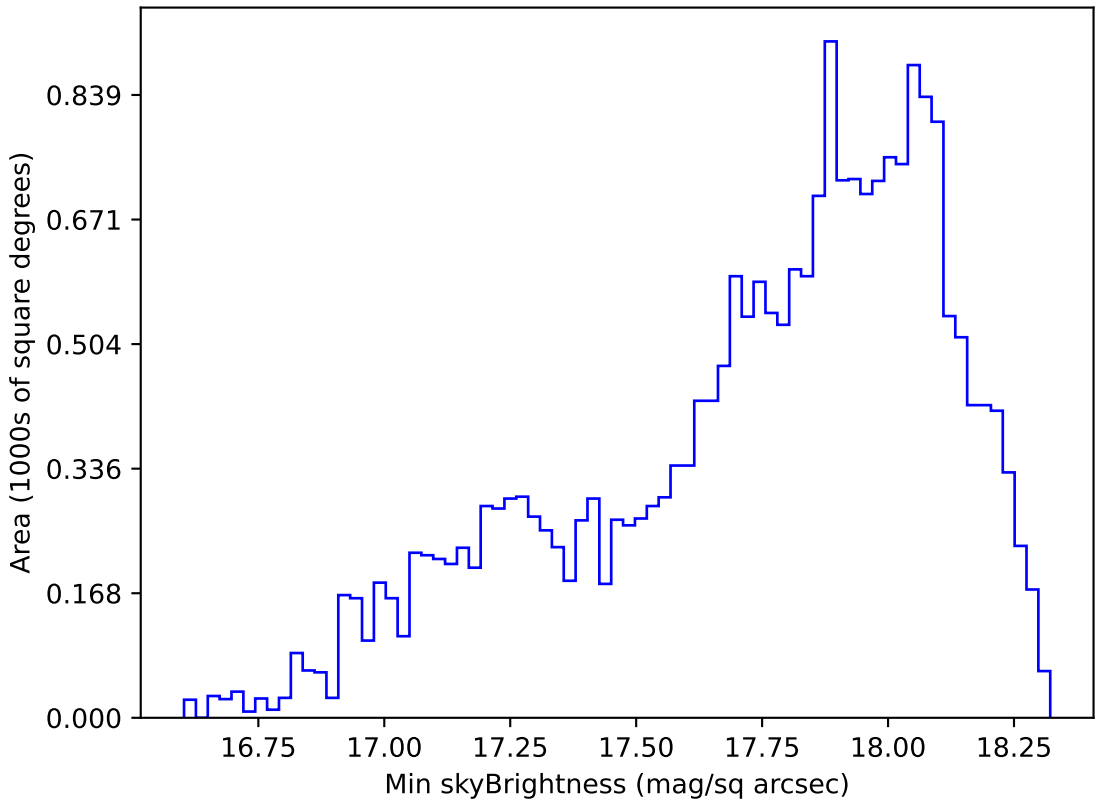
weather_cloudso2v3.4_10yrs Yr 1 y band: Min skyBrightness
