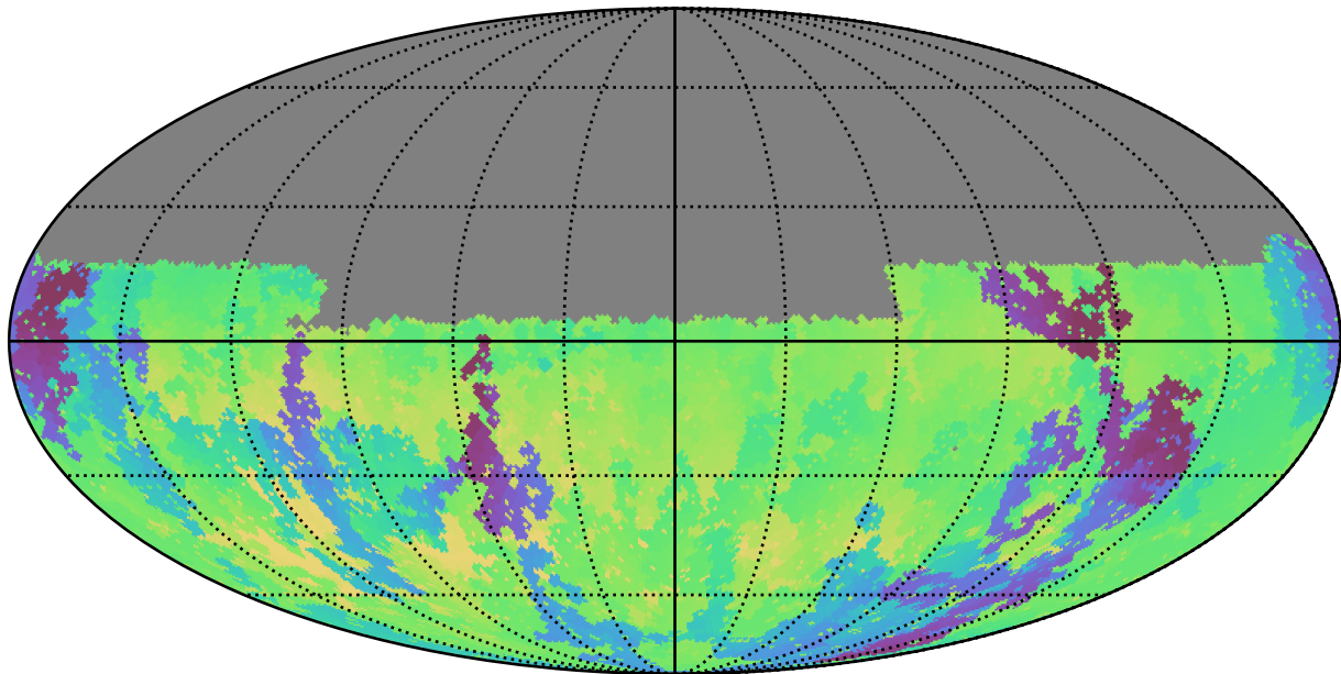
weather_cloudso2v3.4_10yrs Yr 1 u band: Min skyBrightness
