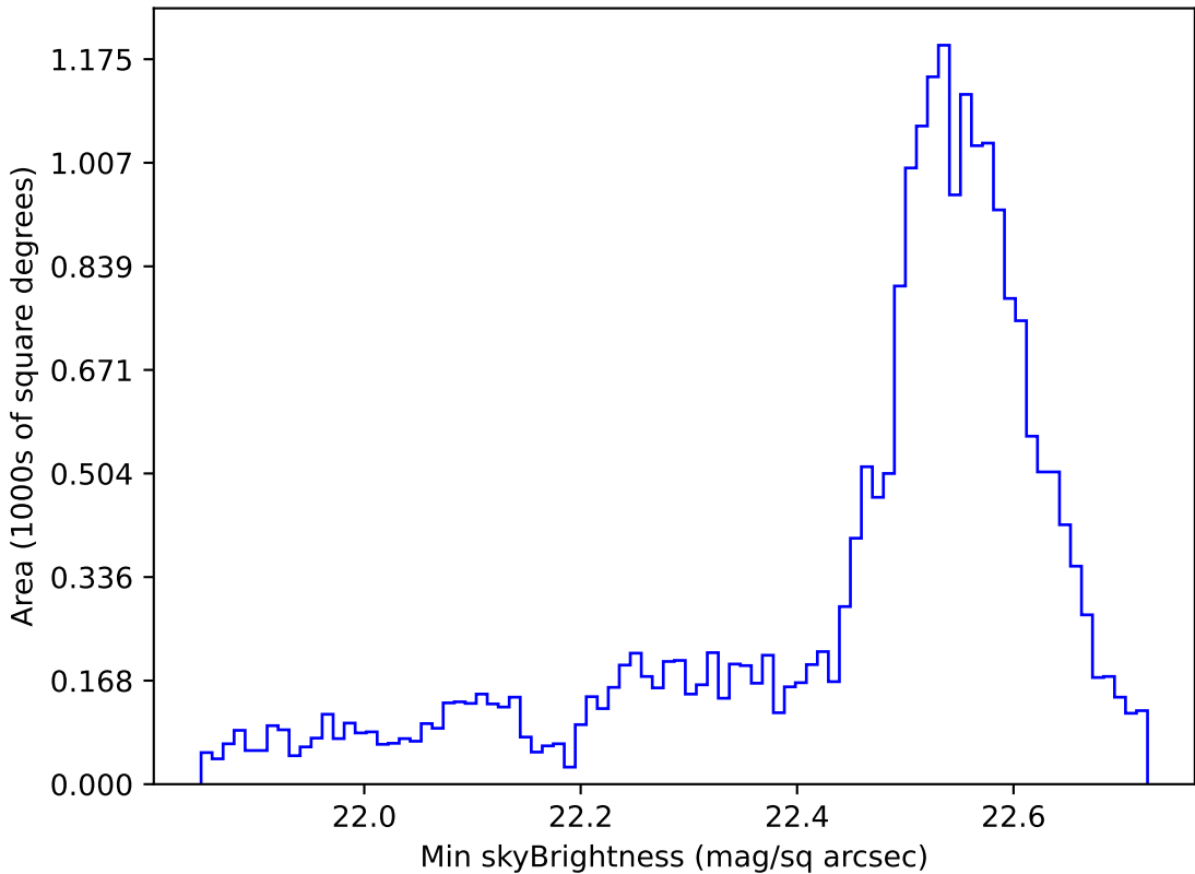
weather_cloudso2v3.4_10yrs Yr 1 u band: Min skyBrightness
