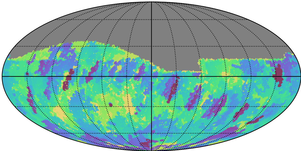
weather_cloudso2v3.4_10yrs Yr 1 r band: Min skyBrightness
