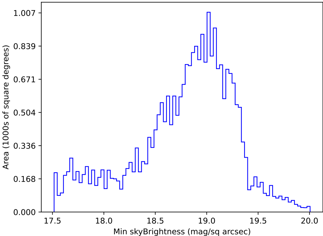
weather_cloudso2v3.4_10yrs Yr 1 i band: Min skyBrightness
