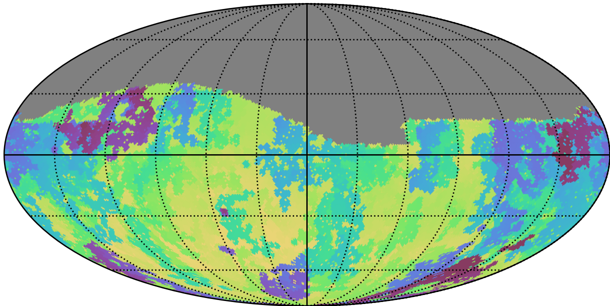
weather_cloudso2v3.4_10yrs Yr 1 g band: Min skyBrightness
