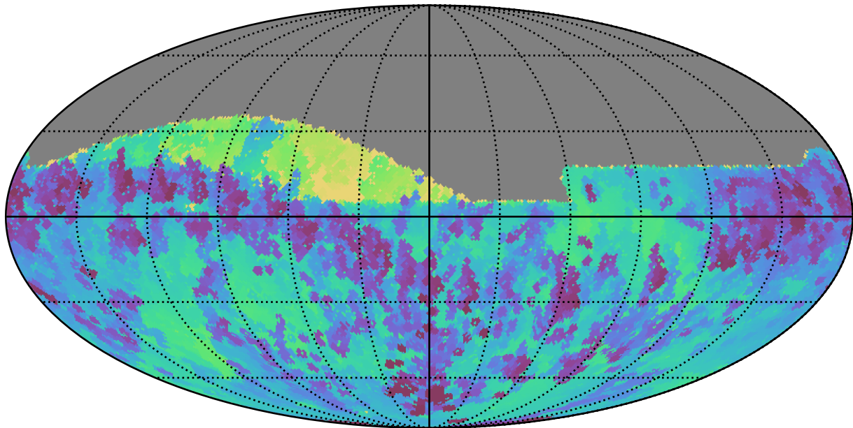
weather_cloudso2v3.4_10yrs Yr 1 all bands: Min skyBrightness
