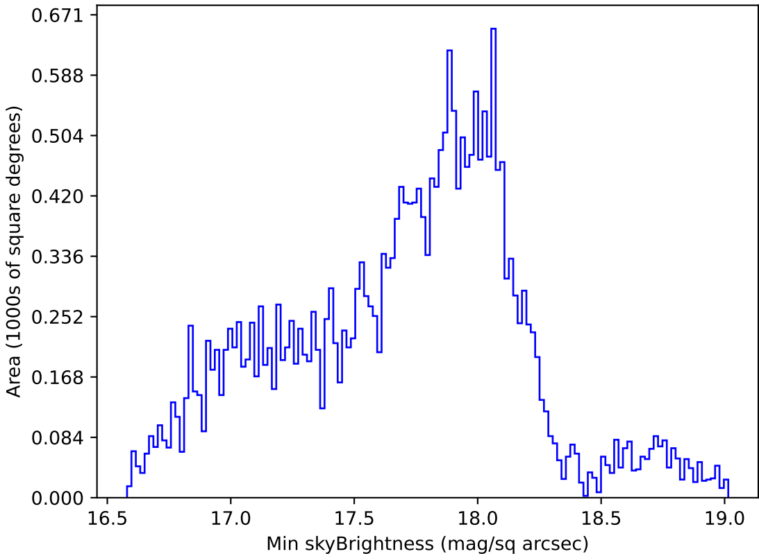
weather_cloudso2v3.4_10yrs Yr 1 all bands: Min skyBrightness
