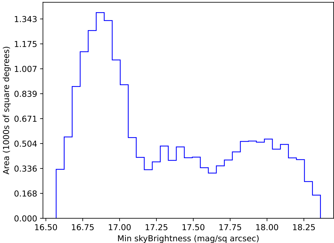
weather_cloudso2v3.4_10yrs WFD z band: Min skyBrightness
