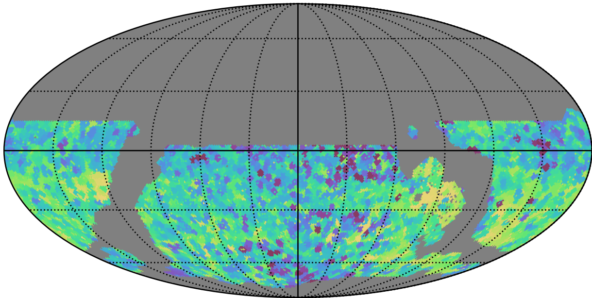
weather_cloudso2v3.4_10yrs WFD y band: Min skyBrightness
