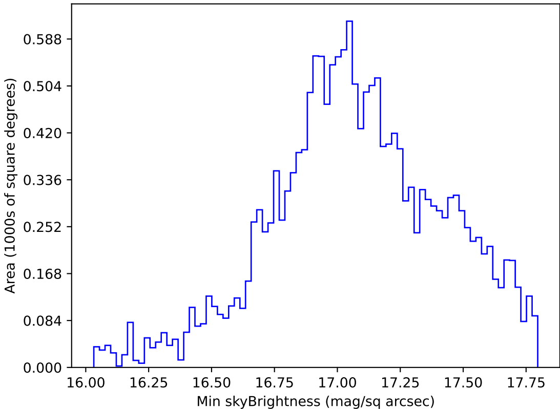
weather_cloudso2v3.4_10yrs WFD y band: Min skyBrightness
