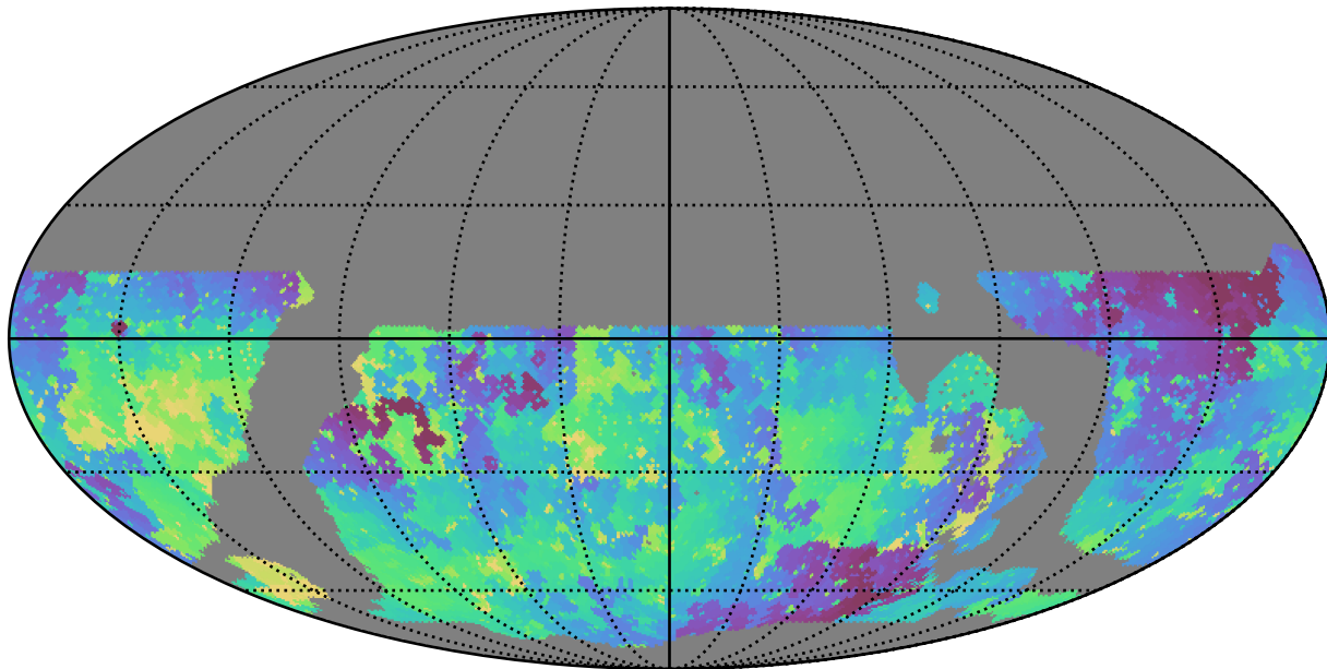
weather_cloudso2v3.4_10yrs WFD u band: Min skyBrightness
