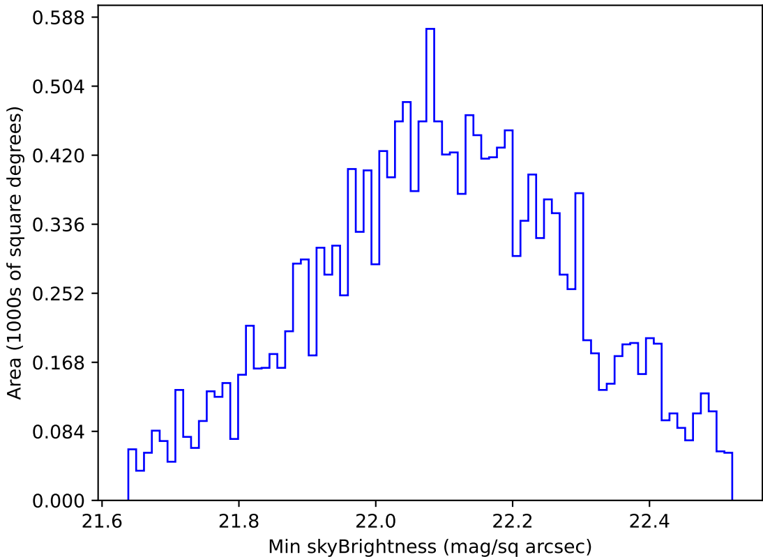
weather_cloudso2v3.4_10yrs WFD u band: Min skyBrightness
