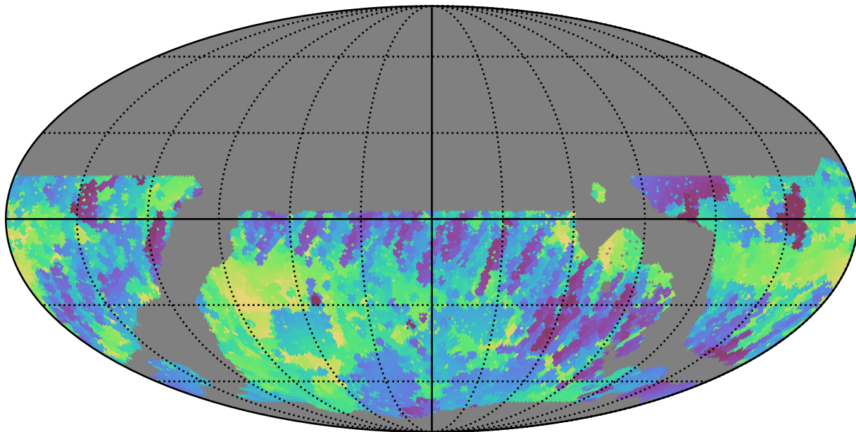
weather_cloudso2v3.4_10yrs WFD r band: Min skyBrightness
