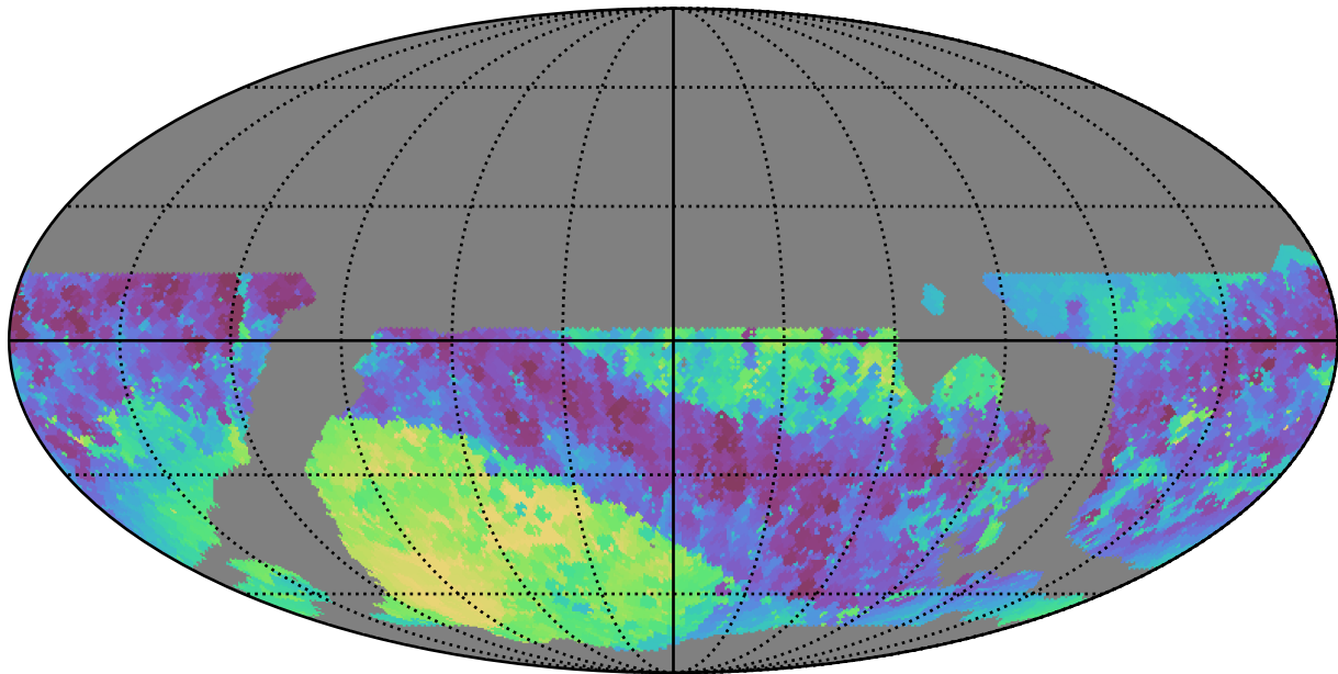
weather_cloudso2v3.4_10yrs WFD i band: Min skyBrightness
