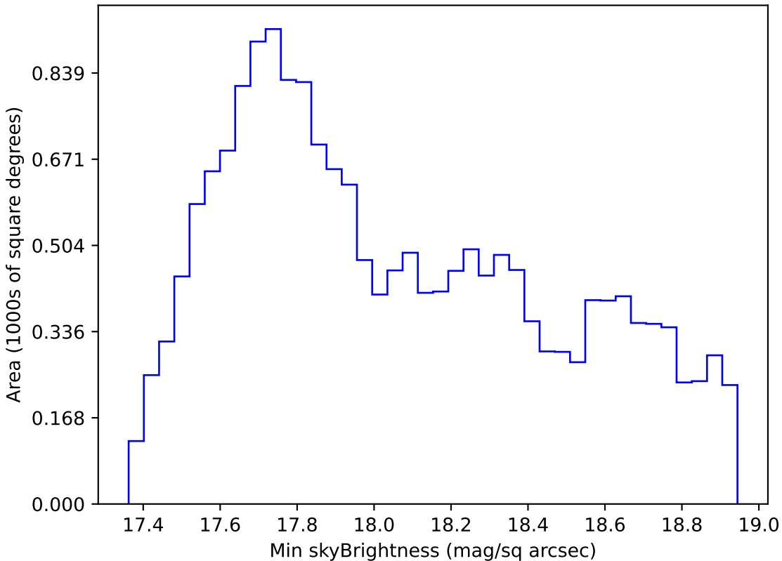
weather_cloudso2v3.4_10yrs WFD i band: Min skyBrightness
