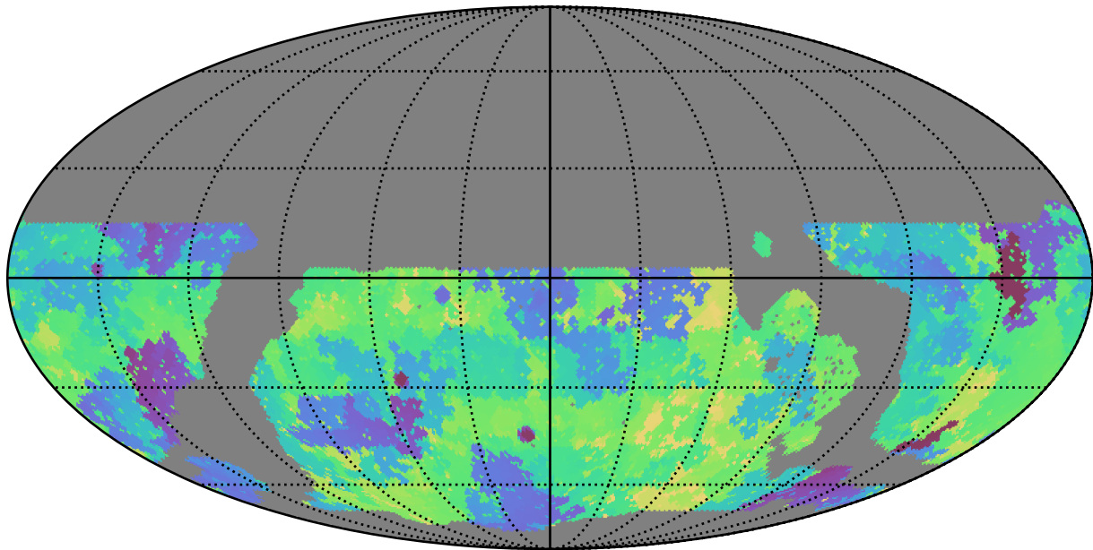
weather_cloudso2v3.4_10yrs WFD g band: Min skyBrightness
