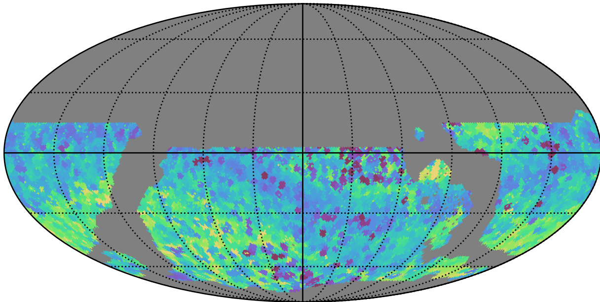
weather_cloudso2v3.4_10yrs WFD all bands: Min skyBrightness
