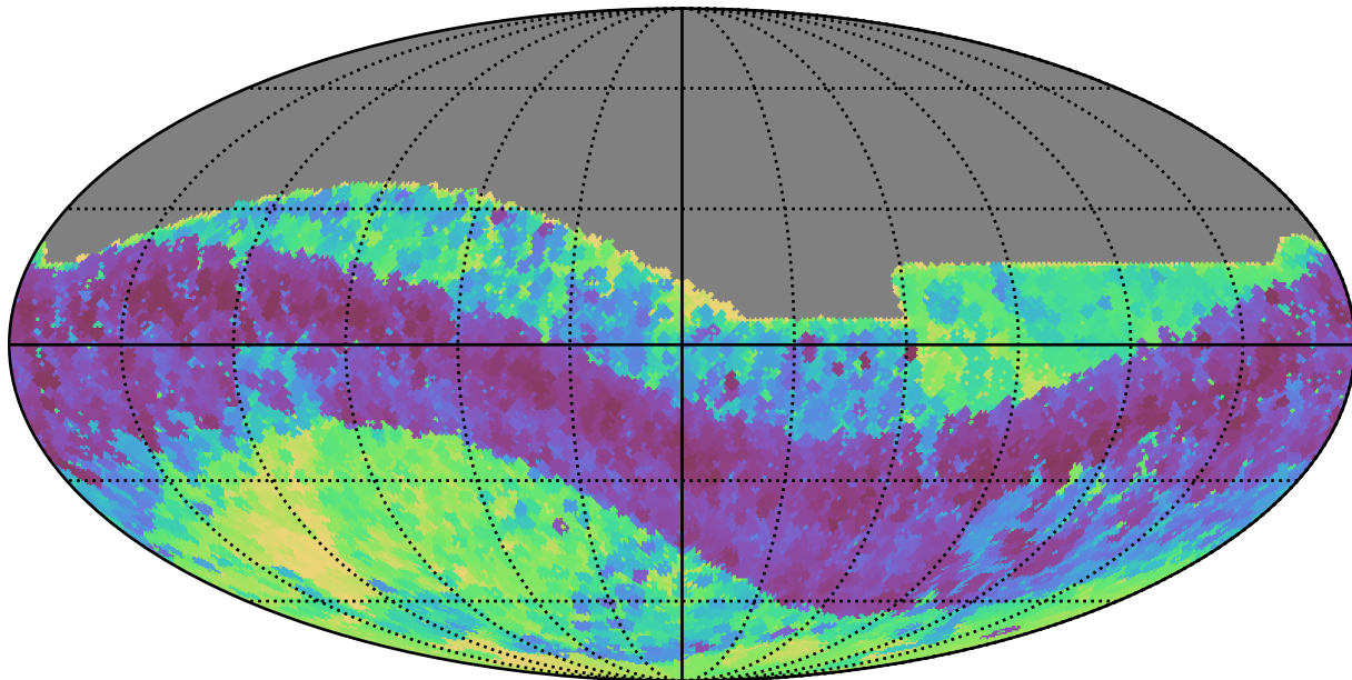
weather_cloudso2v3.4_10yrs All sky z band: Min skyBrightness
