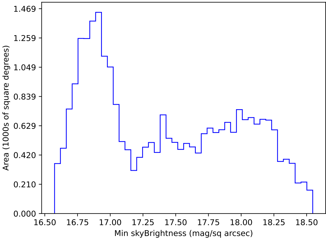
weather_cloudso2v3.4_10yrs All sky z band: Min skyBrightness
