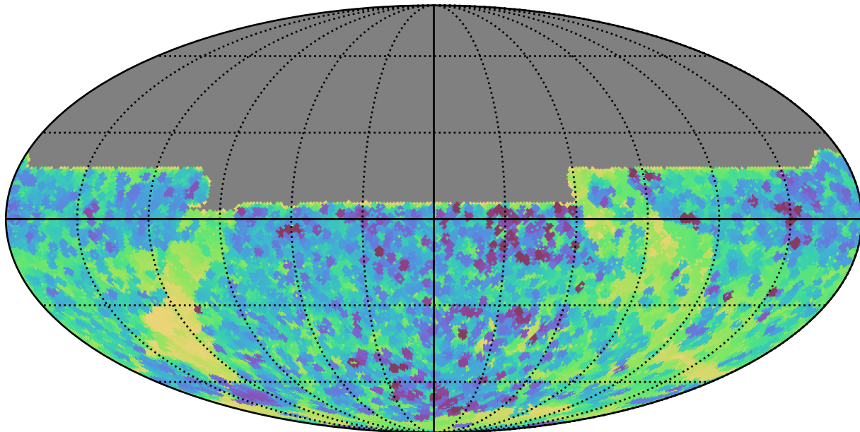
weather_cloudso2v3.4_10yrs All sky y band: Min skyBrightness
