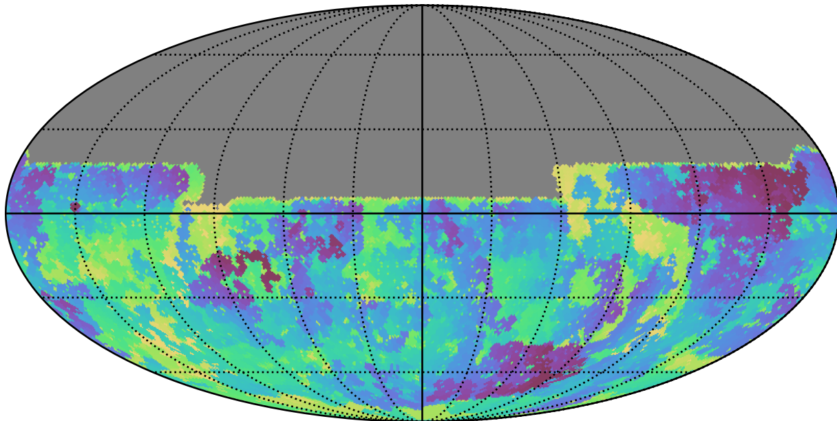
weather_cloudso2v3.4_10yrs All sky u band: Min skyBrightness
