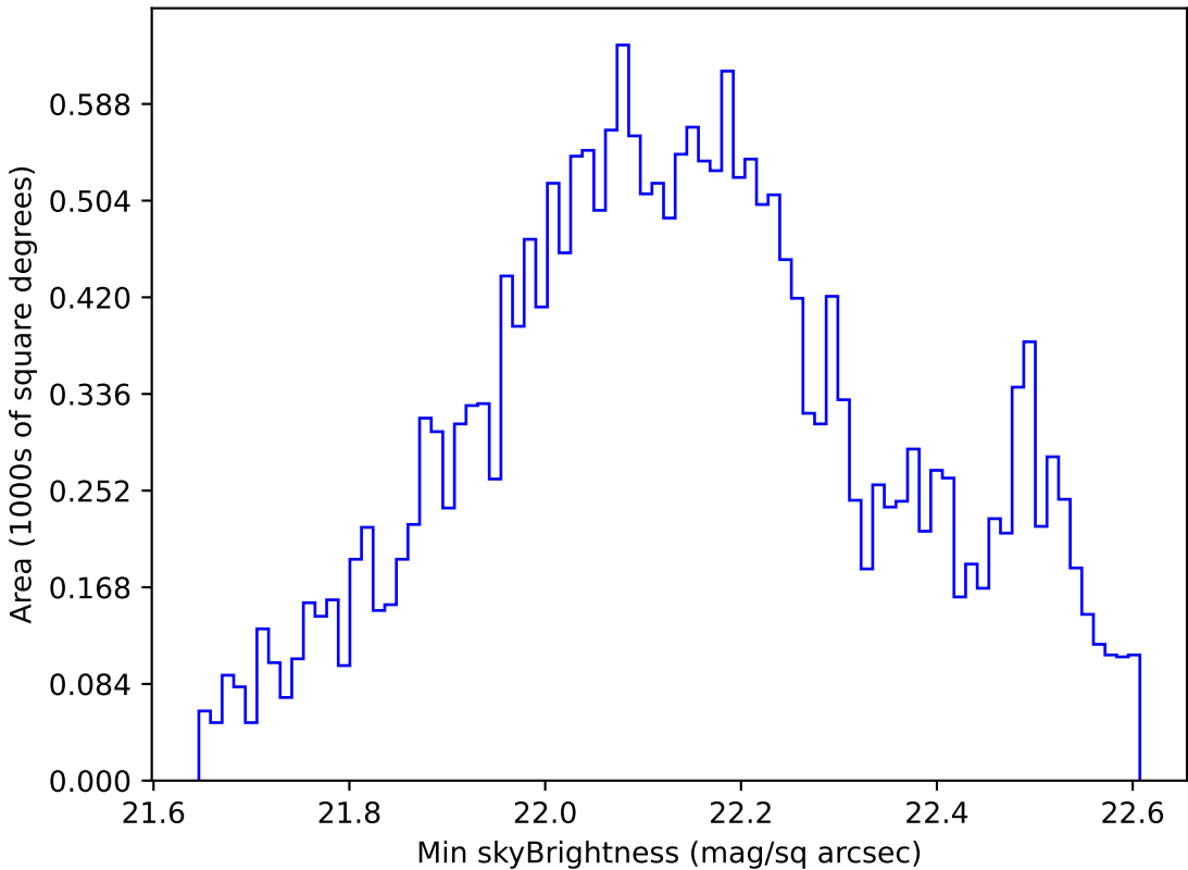
weather_cloudso2v3.4_10yrs All sky u band: Min skyBrightness
