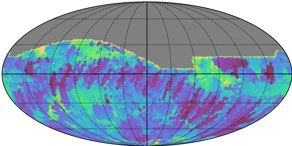
weather_cloudso2v3.4_10yrs All sky r band: Min skyBrightness
