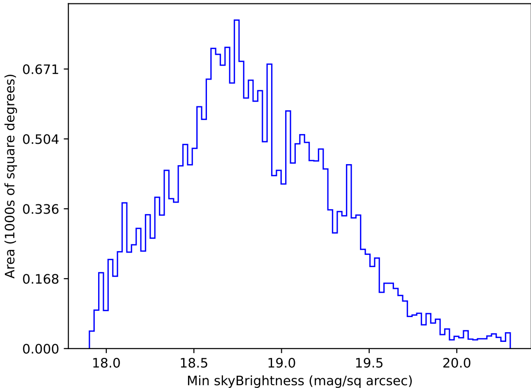
weather_cloudso2v3.4_10yrs All sky r band: Min skyBrightness
