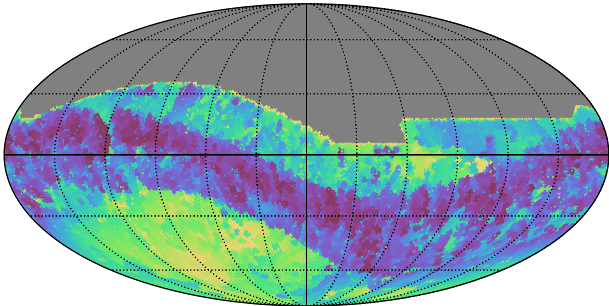
weather_cloudso2v3.4_10yrs All sky i band: Min skyBrightness
