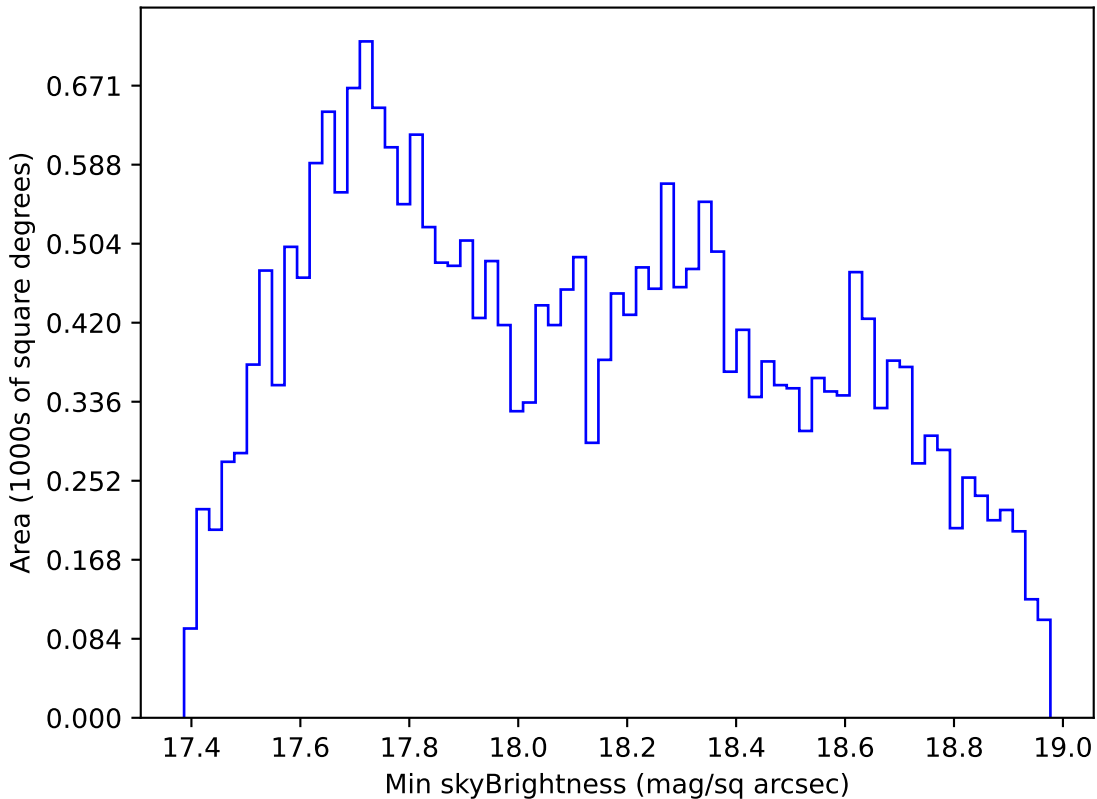
weather_cloudso2v3.4_10yrs All sky i band: Min skyBrightness
