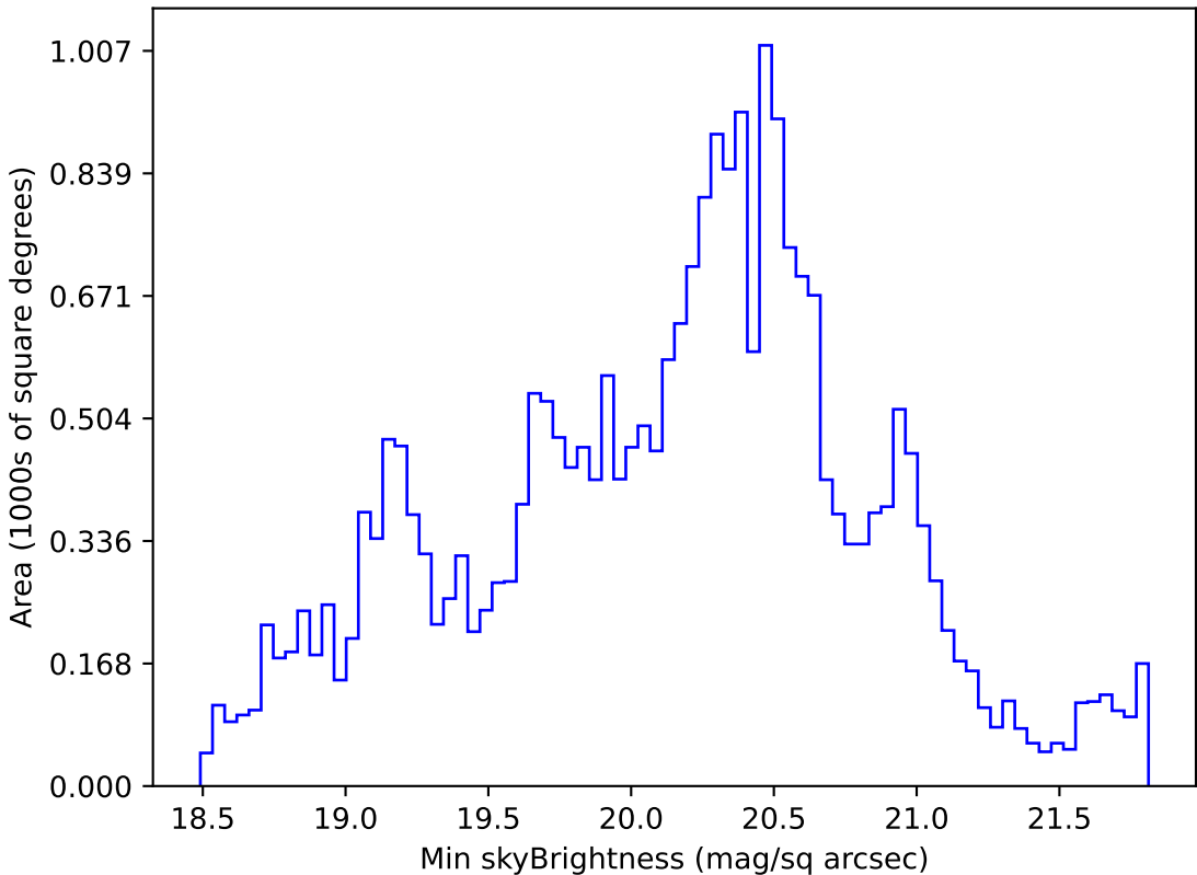
weather_cloudso2v3.4_10yrs All sky g band: Min skyBrightness
