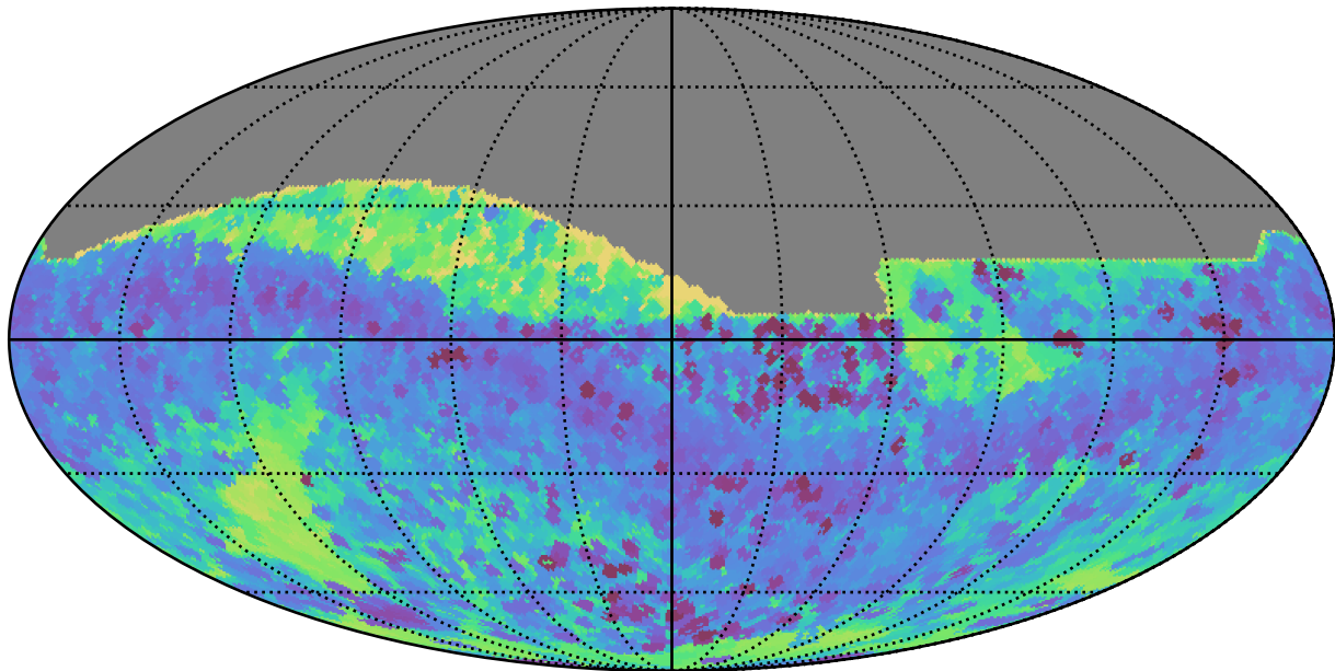
weather_cloudso2v3.4_10yrs All sky all bands: Min skyBrightness
