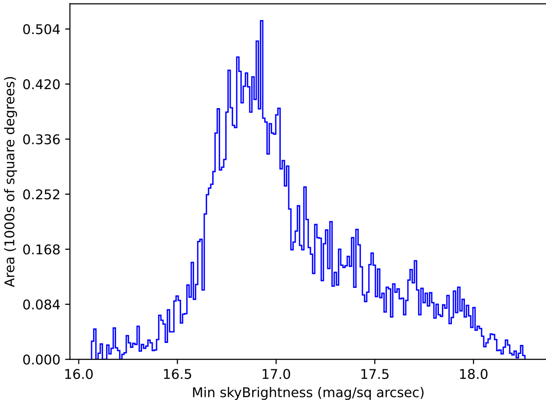
weather_cloudso2v3.4_10yrs All sky all bands: Min skyBrightness
