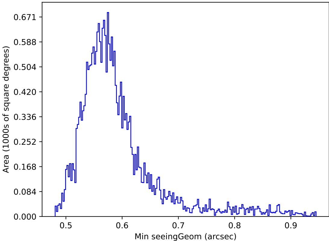
weather_cloudso2v3.4_10yrs Yr 1 all bands: Min seeingGeom
