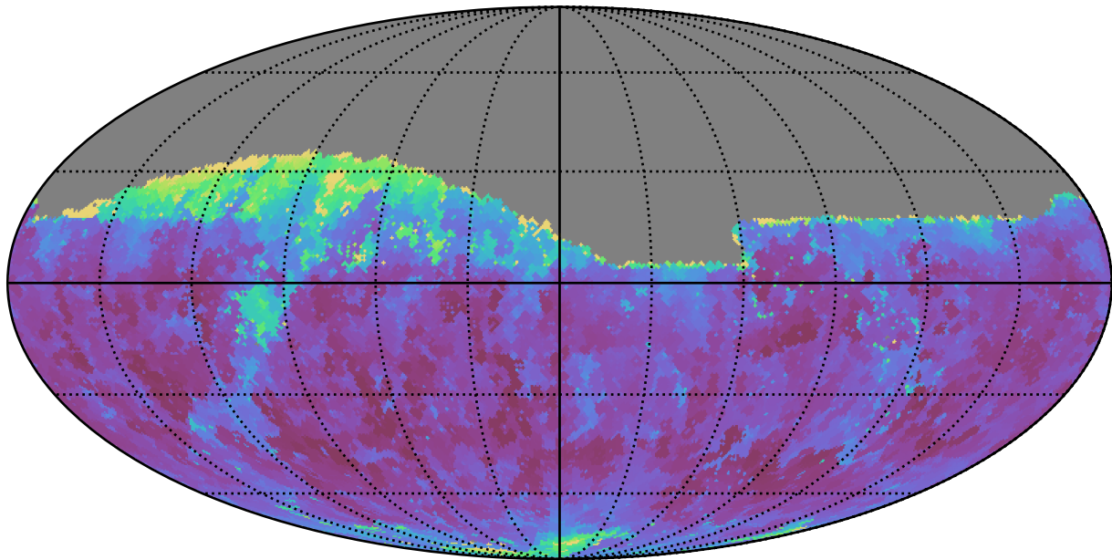
weather_cloudso2v3.4_10yrs Yr 1 z band: Min seeingEff
