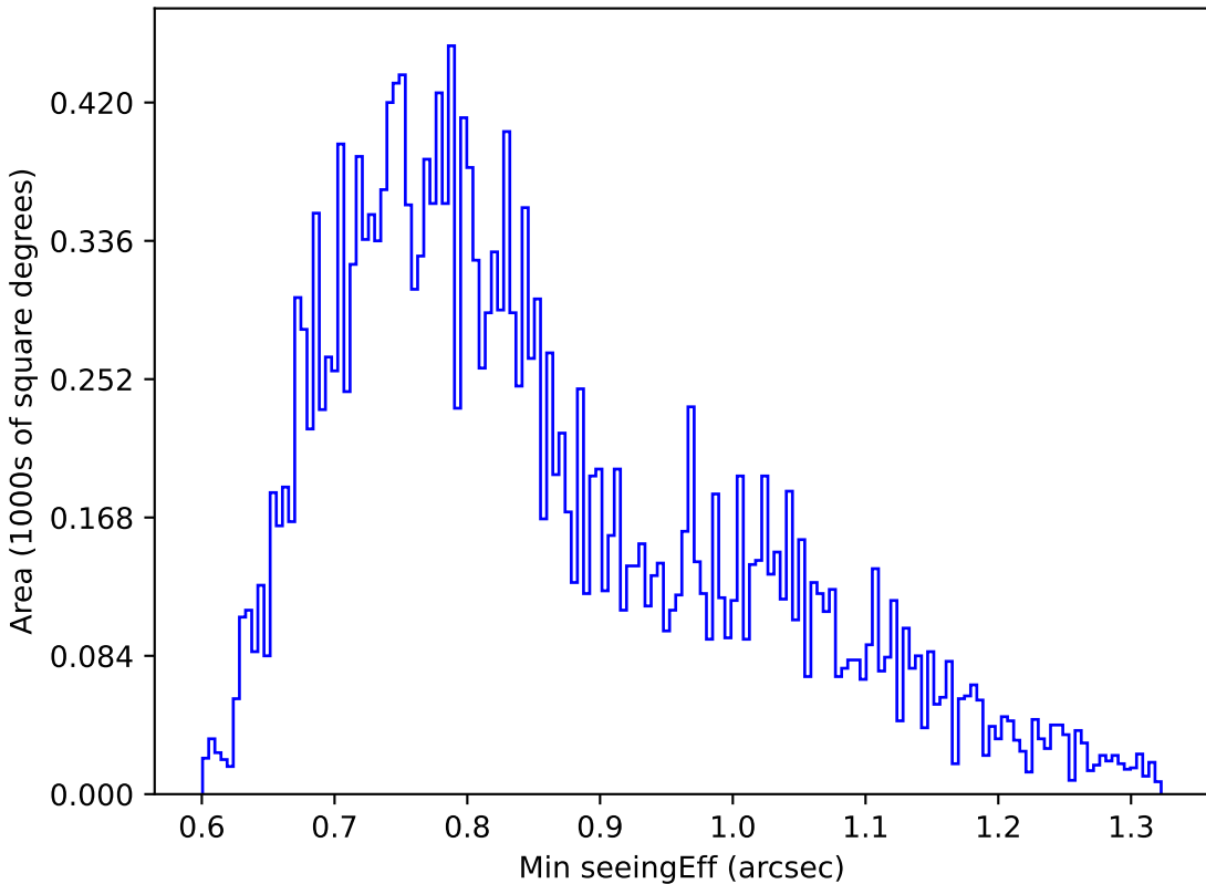
weather_cloudso2v3.4_10yrs Yr 1 u band: Min seeingEff
