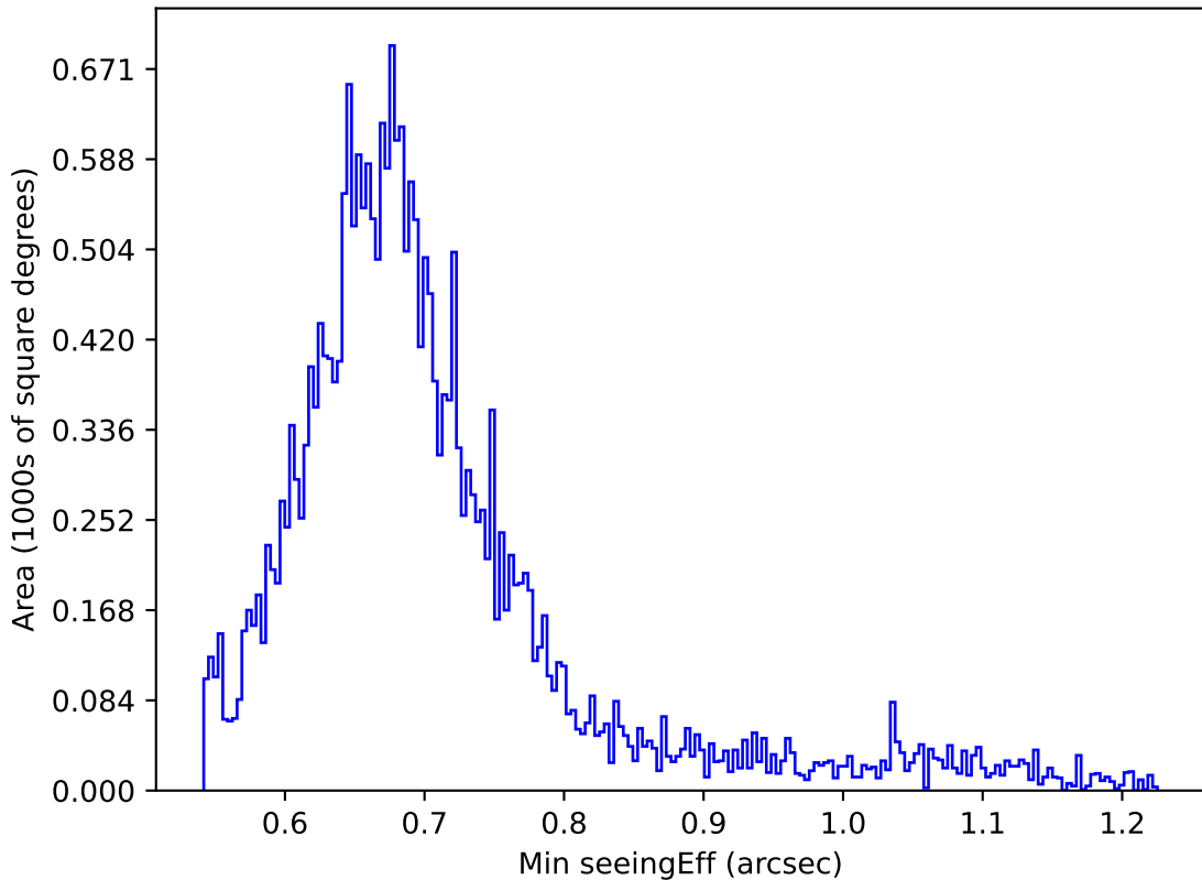
weather_cloudso2v3.4_10yrs Yr 1 r band: Min seeingEff
