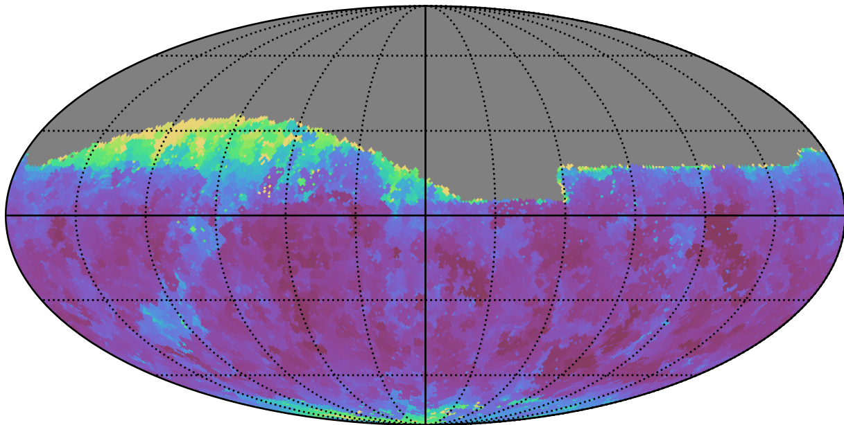
weather_cloudso2v3.4_10yrs Yr 1 i band: Min seeingEff
