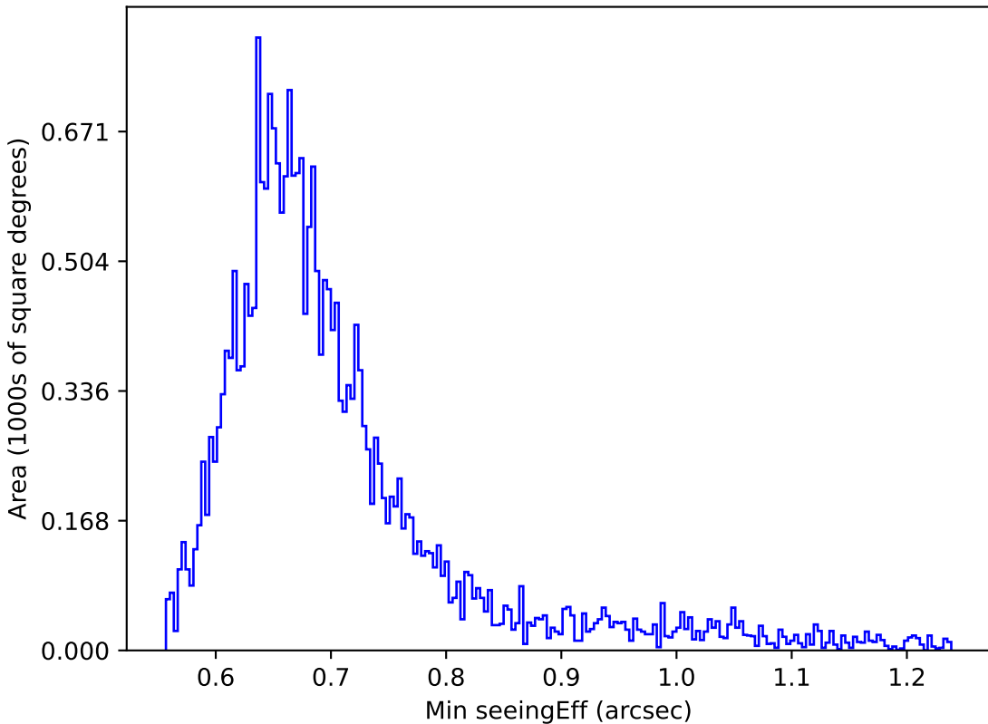
weather_cloudso2v3.4_10yrs Yr 1 i band: Min seeingEff
