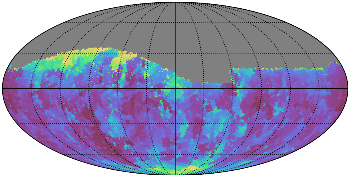
weather_cloudso2v3.4_10yrs Yr 1 g band: Min seeingEff
