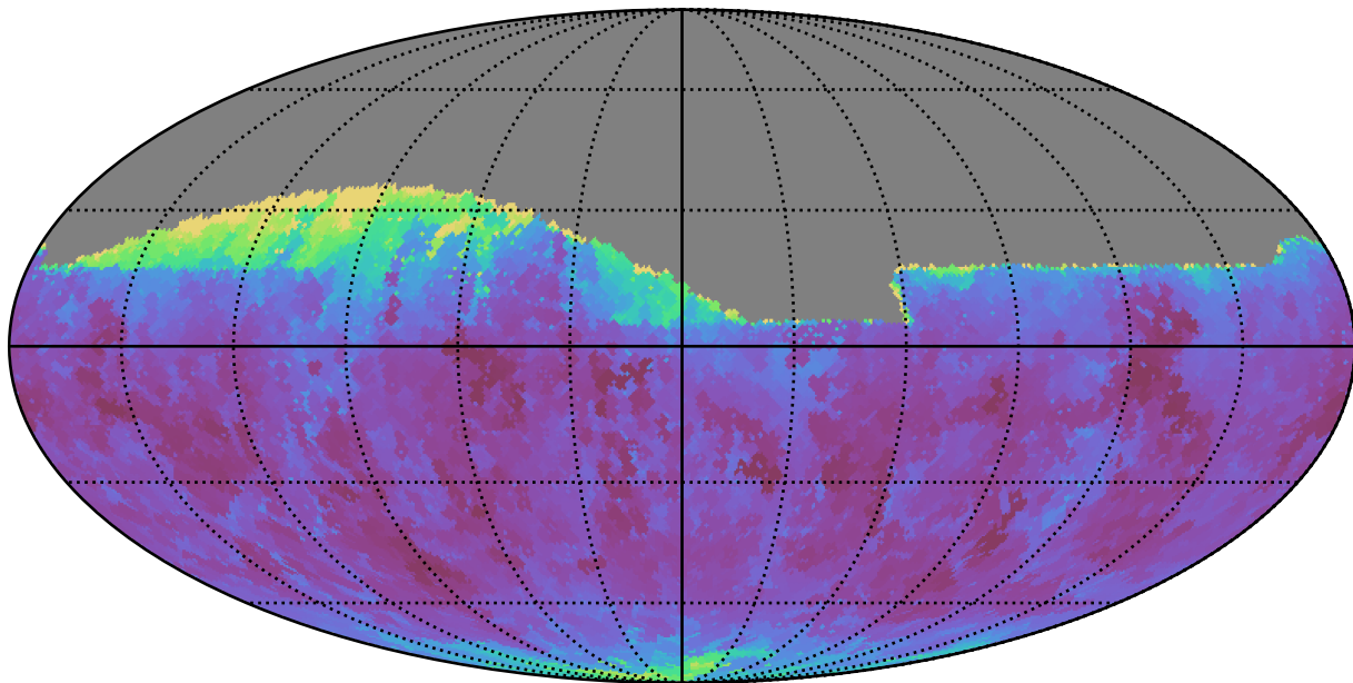
weather_cloudso2v3.4_10yrs Yr 1 all bands: Min seeingEff
