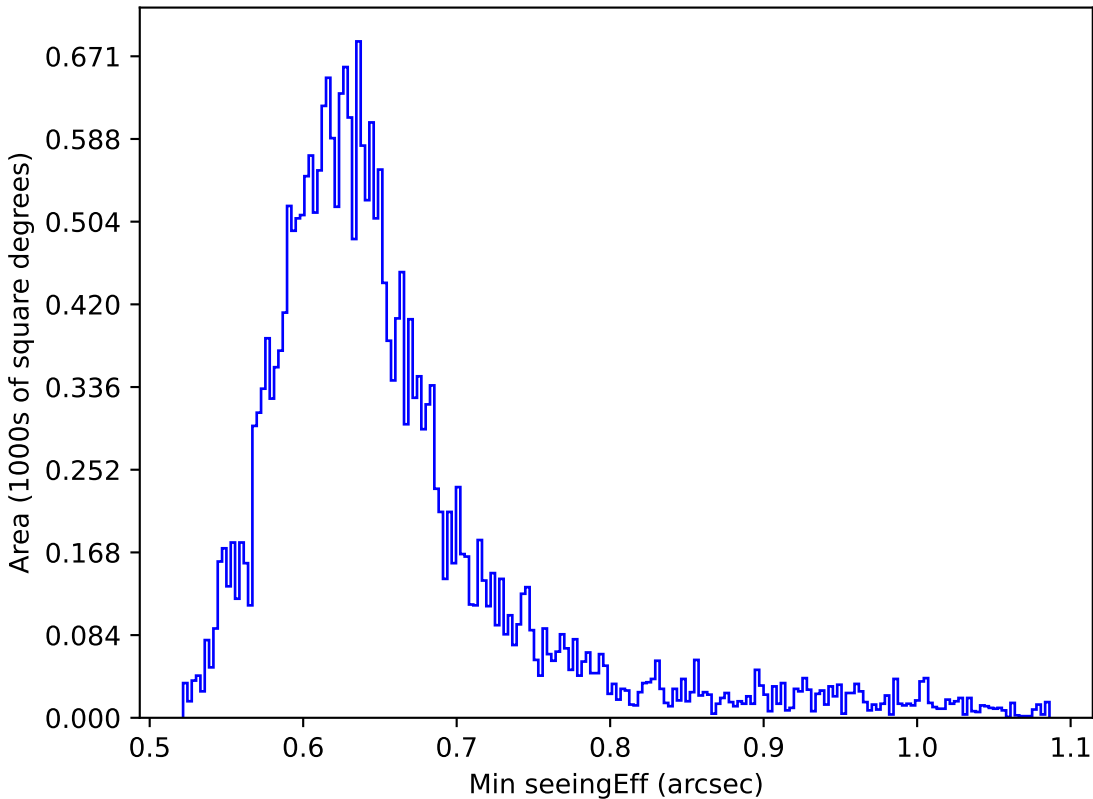
weather_cloudso2v3.4_10yrs Yr 1 all bands: Min seeingEff
