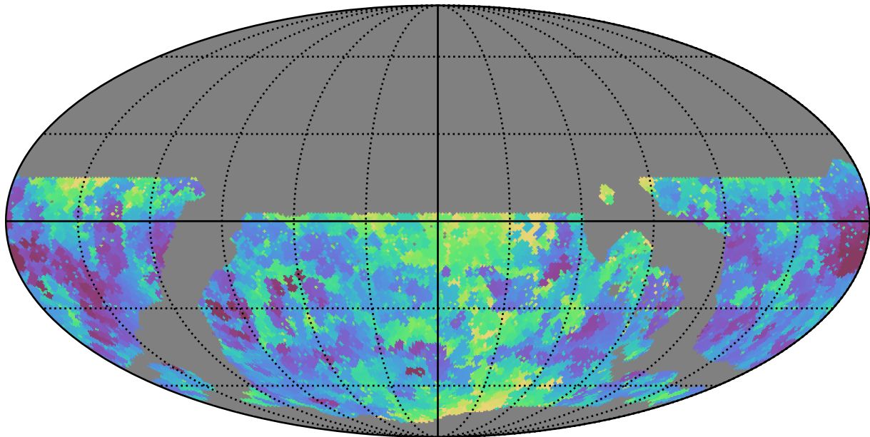
weather_cloudso2v3.4_10yrs WFD u band: Min seeingEff
