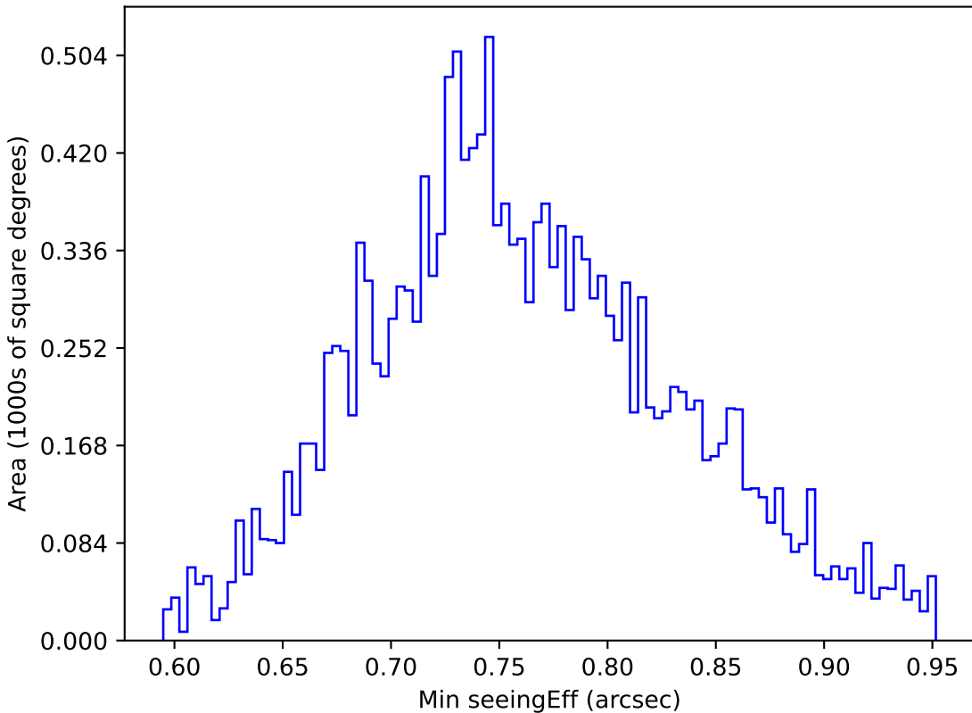
weather_cloudso2v3.4_10yrs WFD u band: Min seeingEff
