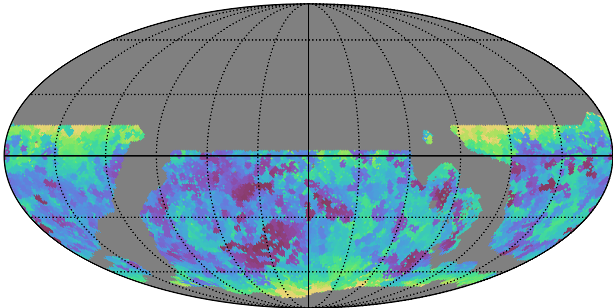
weather_cloudso2v3.4_10yrs WFD all bands: Min seeingEff
