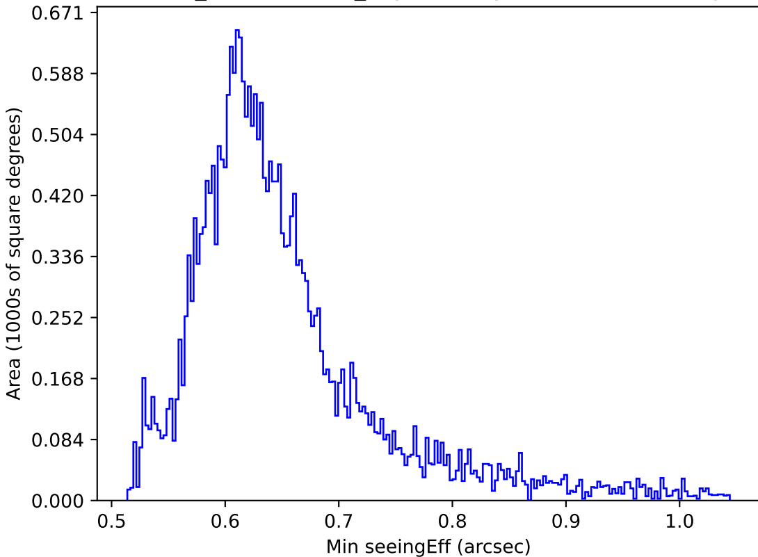
weather_cloudso2v3.4_10yrs All sky z band: Min seeingEff
