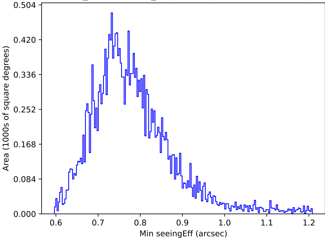
weather_cloudso2v3.4_10yrs All sky u band: Min seeingEff
