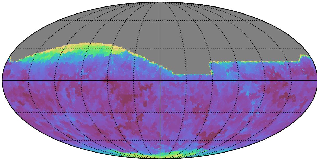
weather_cloudso2v3.4_10yrs All sky r band: Min seeingEff
