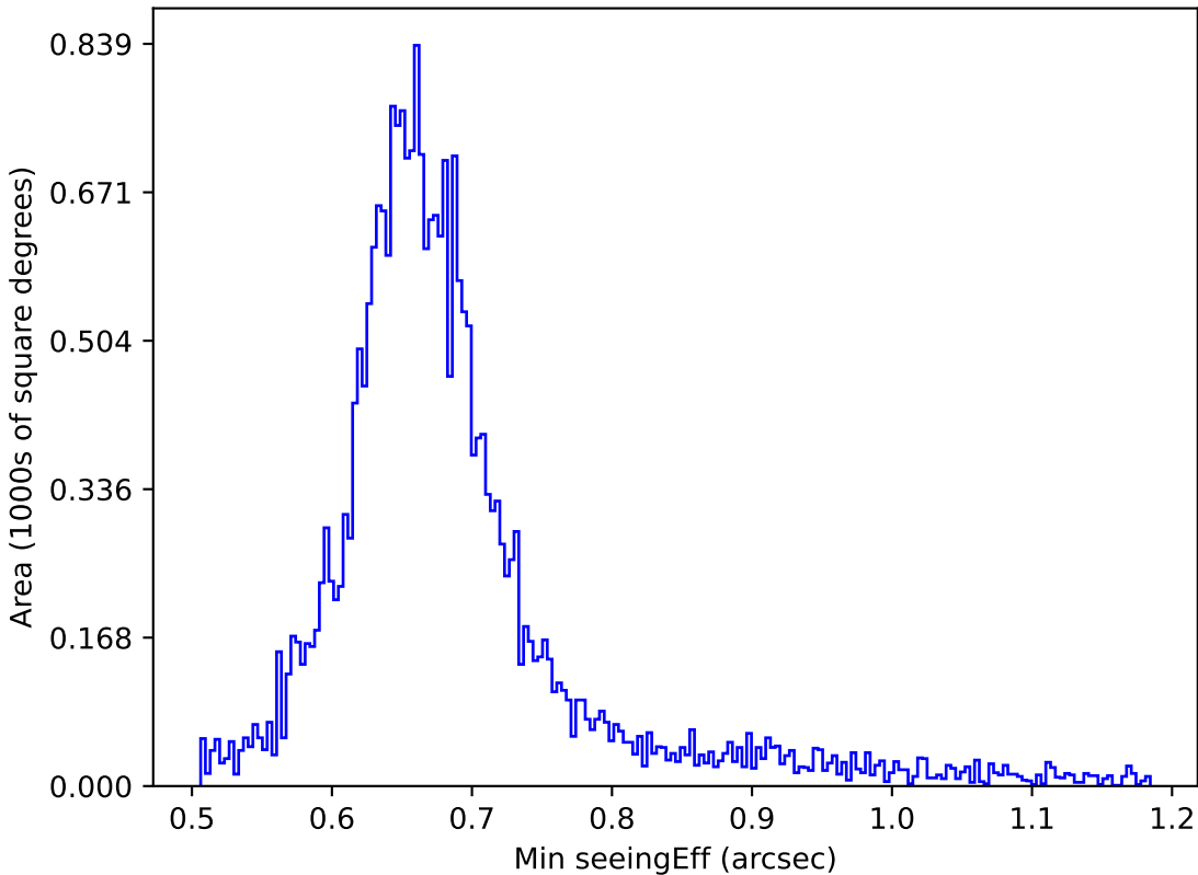
weather_cloudso2v3.4_10yrs All sky g band: Min seeingEff
