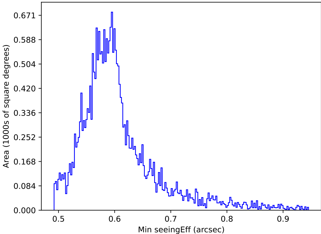
weather_cloudso2v3.4_10yrs All sky all bands: Min seeingEff
