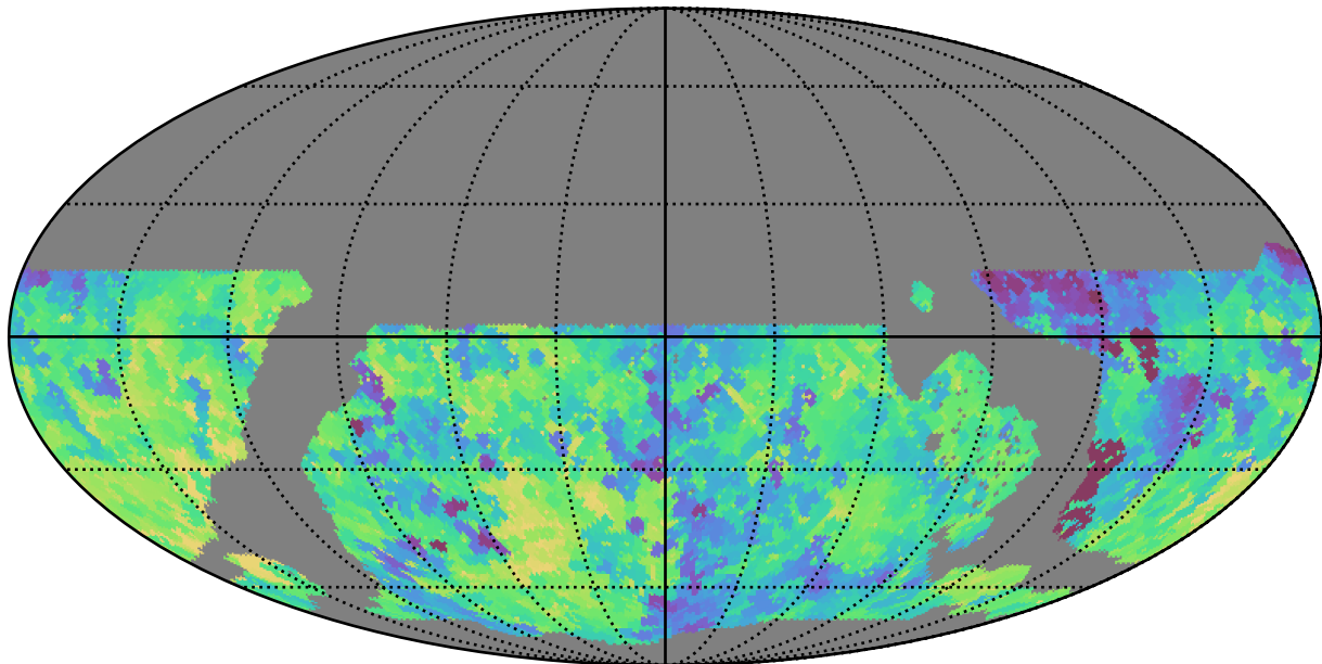
weather_cloudso2v3.4_10yrs WFD all bands: Min saturation_mag
