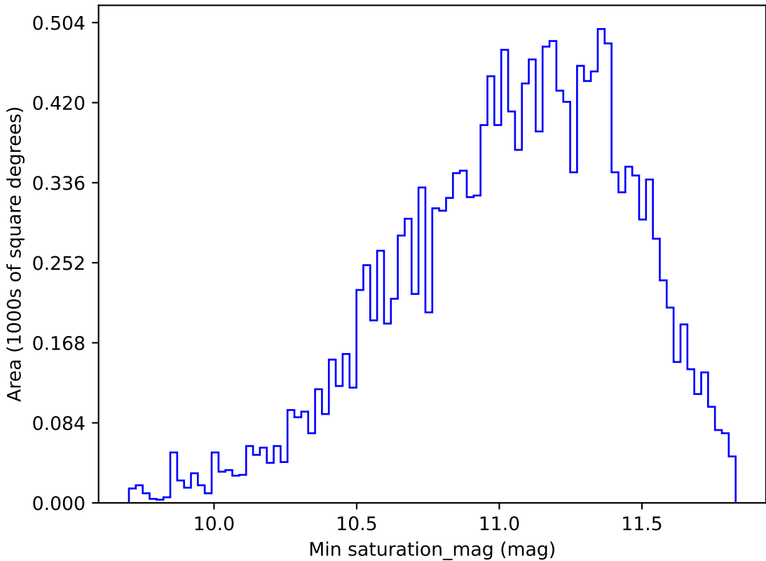
weather_cloudso2v3.4_10yrs WFD all bands: Min saturation_mag
